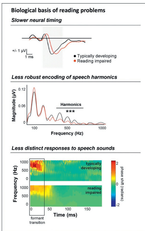
Fig. 12.7. Reading problems are associated with deficits in the neural encoding of sound. Many of the same aspects of sound processing that are deficient in populations with language-based impairments are strengthened in auditory experts such as musicians. (For review, see Tierney and Kraus, 2013b.)
