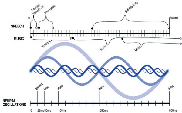
Fig. 12.1. Timescales of speech and music characteristics: different frequencies of neural oscillatory activity lock on to meaningful temporal patterns in speech and music.
